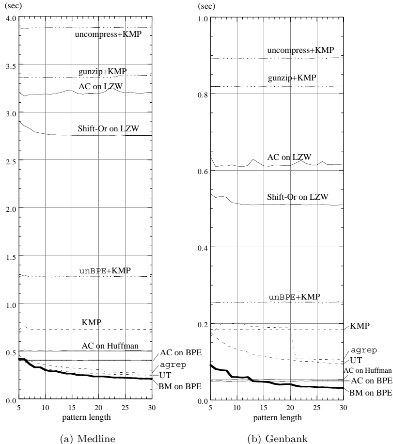
Fig. 12 Running times (in CPU time).
