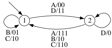
Fig. 3 Finite-state encoder with two states.
