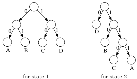
Fig. 4 Code-trees.
